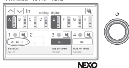
DIGITAL TD CONTROLLER NXAMP4x2 MK2
