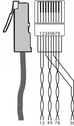
Figure 4: CAT 5 PINOUT
